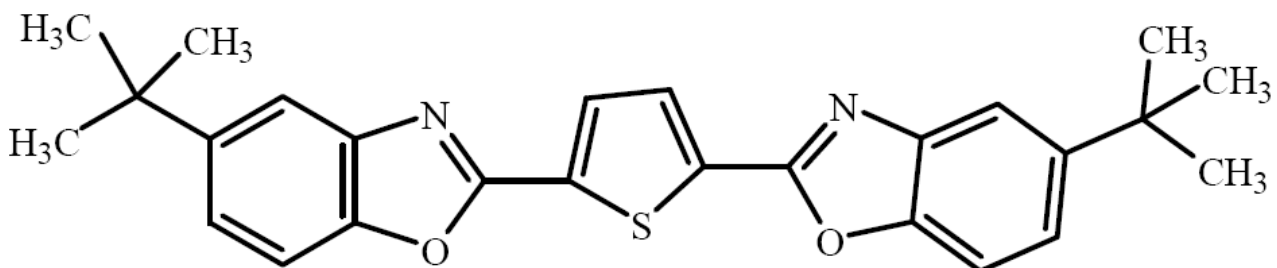
MCA ® Brightener OB-184 for plastics and coatings
